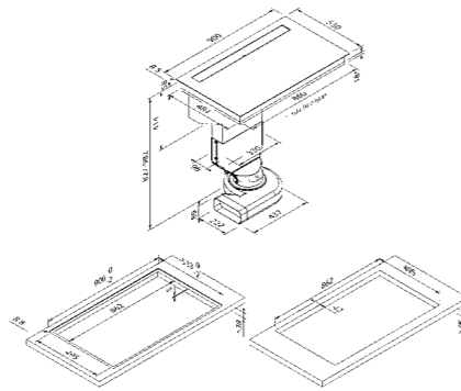
Stand-alone hob, integrated extractor fan
